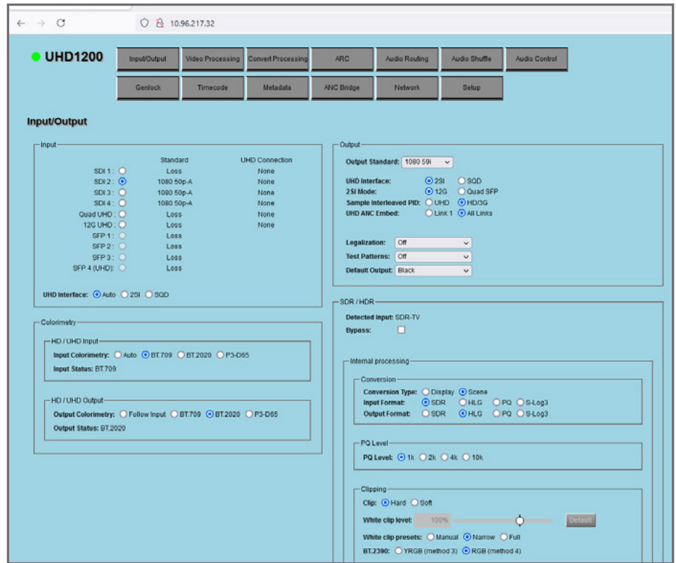
HTML5 web interface for UHD1200
